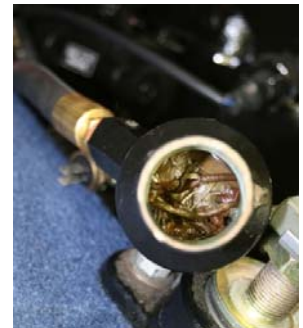
Without a weed strainer fitted, Trans Coolers can be blocked by weed and debris
